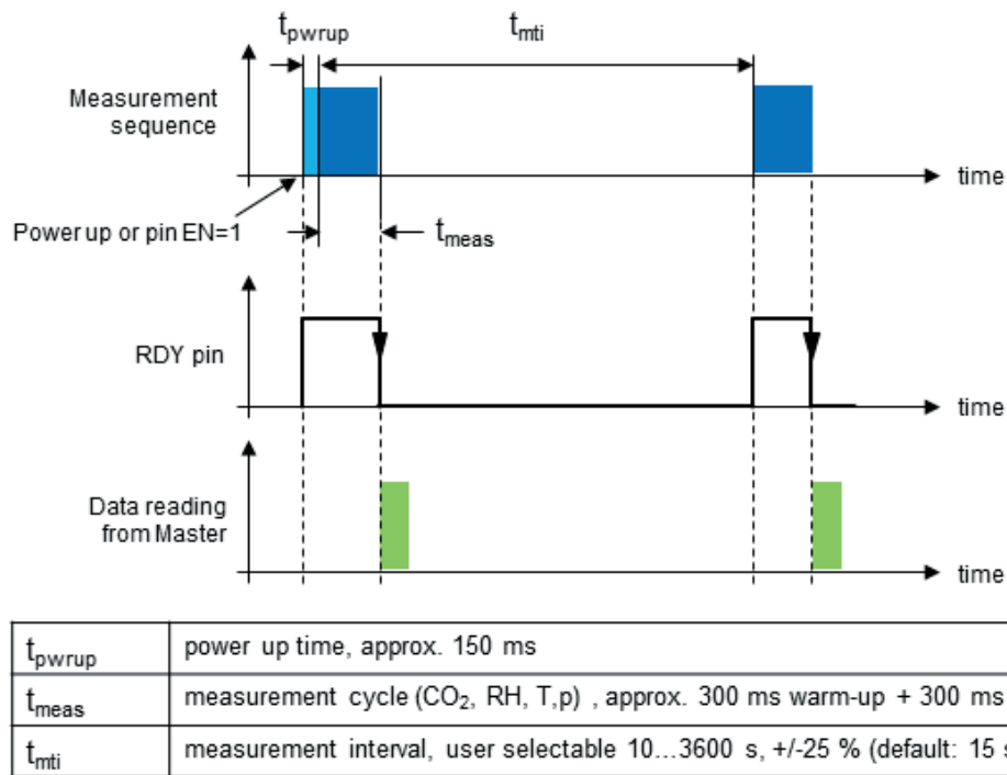
Fig. 7 Timing details (see chapter 4.4.3: "CO 2 Parameter Settings")
