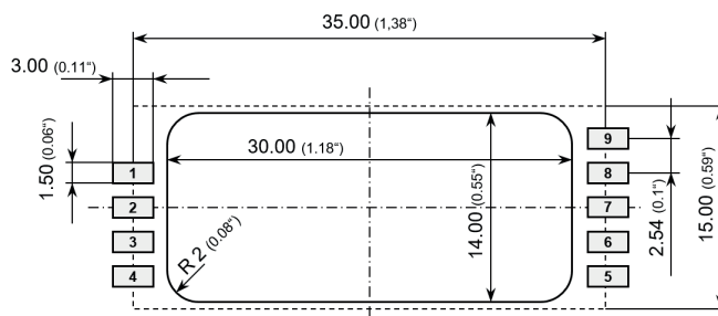
Fig. 2 Recommended PCB footprint
