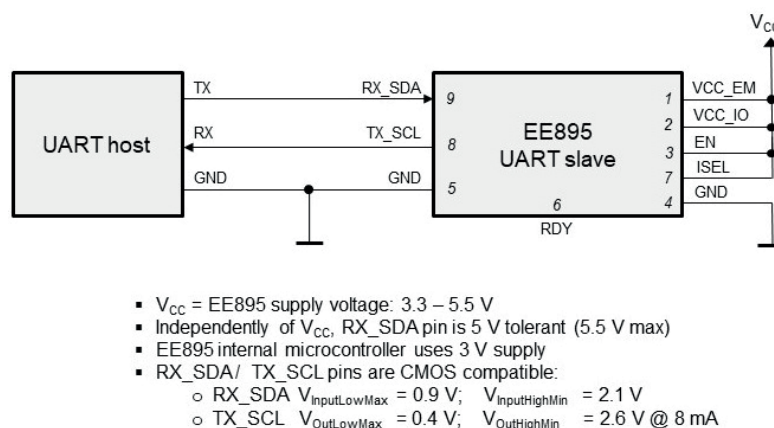
Fig. 9 Example UART interface
